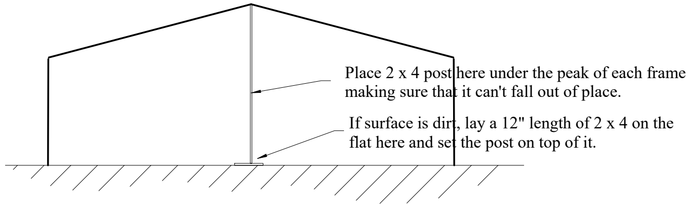
Carport without Gusset
